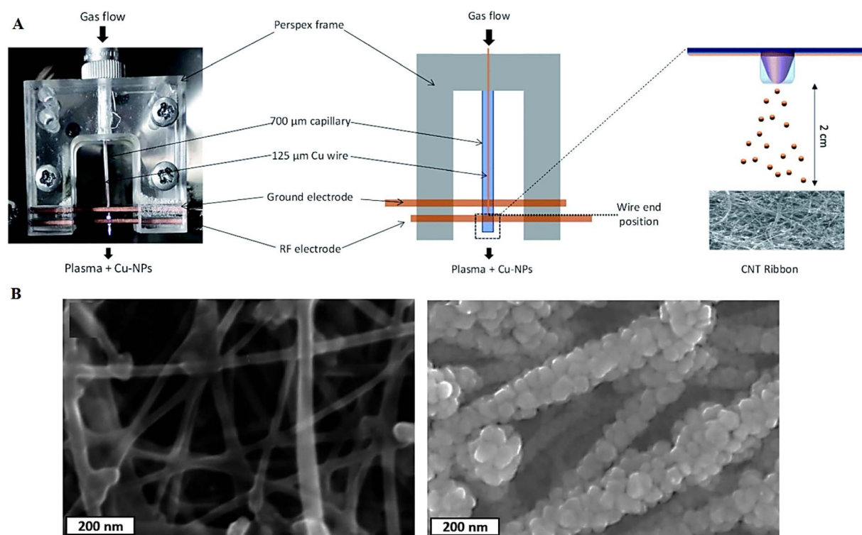
Fig. 2 (A) The preparative process of Cu NPs and carbon nanotubes/Cu-NP composites based on the microplasma process. (B) Scanning electron microscopy (SEM) images of (left) pristine carbon nanotube ribbons and (right) decorated carbon nanotube/Cu-NP composites. Adapted from ref. 70 with permission. Copyright 2021 Royal Society of Chemistry (CC BY).
