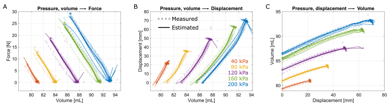
Fig. 5 Mapping between the pressure, volume, force, and displacement, for three-point bending. The round markers correspond to ground-truth values and the continuous curves represent estimated values from the neural networks. The different colours represent the initial pressure value at zero displacement. (A) Mapping from pressure and volume to force, (B) mapping from pressure and volume to displacement, (C) mapping from pressure and displacement to volume.
