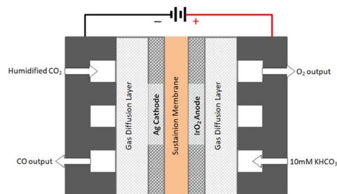
Fig. 5 Schematics of a typical membrane electrode assembly (MEA) cell for CO 2 electroconversion to CO (reproduced from Liu et al. , 2018). 34
