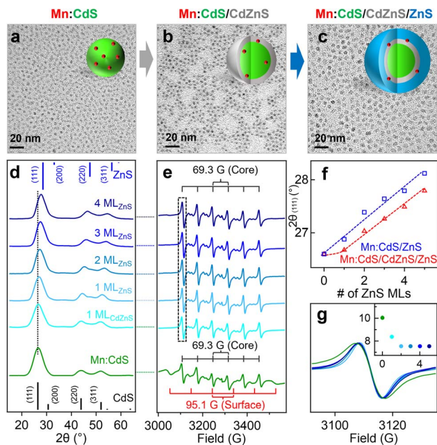
Fig. 1 (a–c) TEM images of Mn:CdS core, Mn:CdS/CdZnS core/shell, and Mn:CdS/CdZnS/ZnS 4 MLs core/multi-shell QDs. (d) XRD patterns and (e) X-band EPR spectra of Mn:CdS/CdZnS/ZnS (1–4 MLs) core/multi-shell QDs. (f) The (111) diffraction peak position of the Mn:CdS/ZnS and Mn:CdS/CdZnS/ZnS core/multi-shell QDs as a function of the ZnS shell thickness. (g) The representative first sextet EPR hyperfine peak to display decreasing spectral linewidth with increasing shell thickness, inset shows the EPR hyperfine peak linewidth (in G) as a function of shell monolayers.
