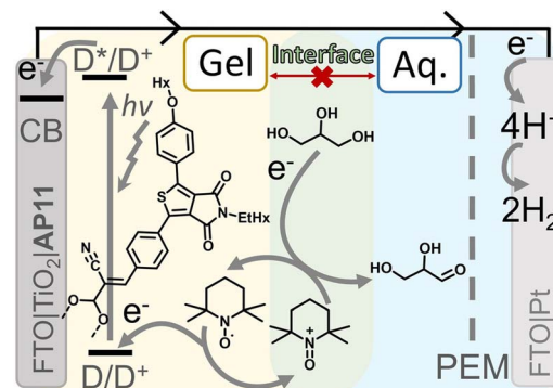
Fig. 29 Photoelectrochemical cell for glycerol oxidation and simultaneous \text{H}_2 evolution proposed by Reek and co-workers. At the photoanode, the yellow and azure colours represent the redox-gel layer and the aqueous solution, respectively, while oxidation of glycerol by oxoammonium \text{TEMPO}^+ occurs at the interface (green area). Reprinted from ref. 156 with permission from Wiley, copyright 2022.
