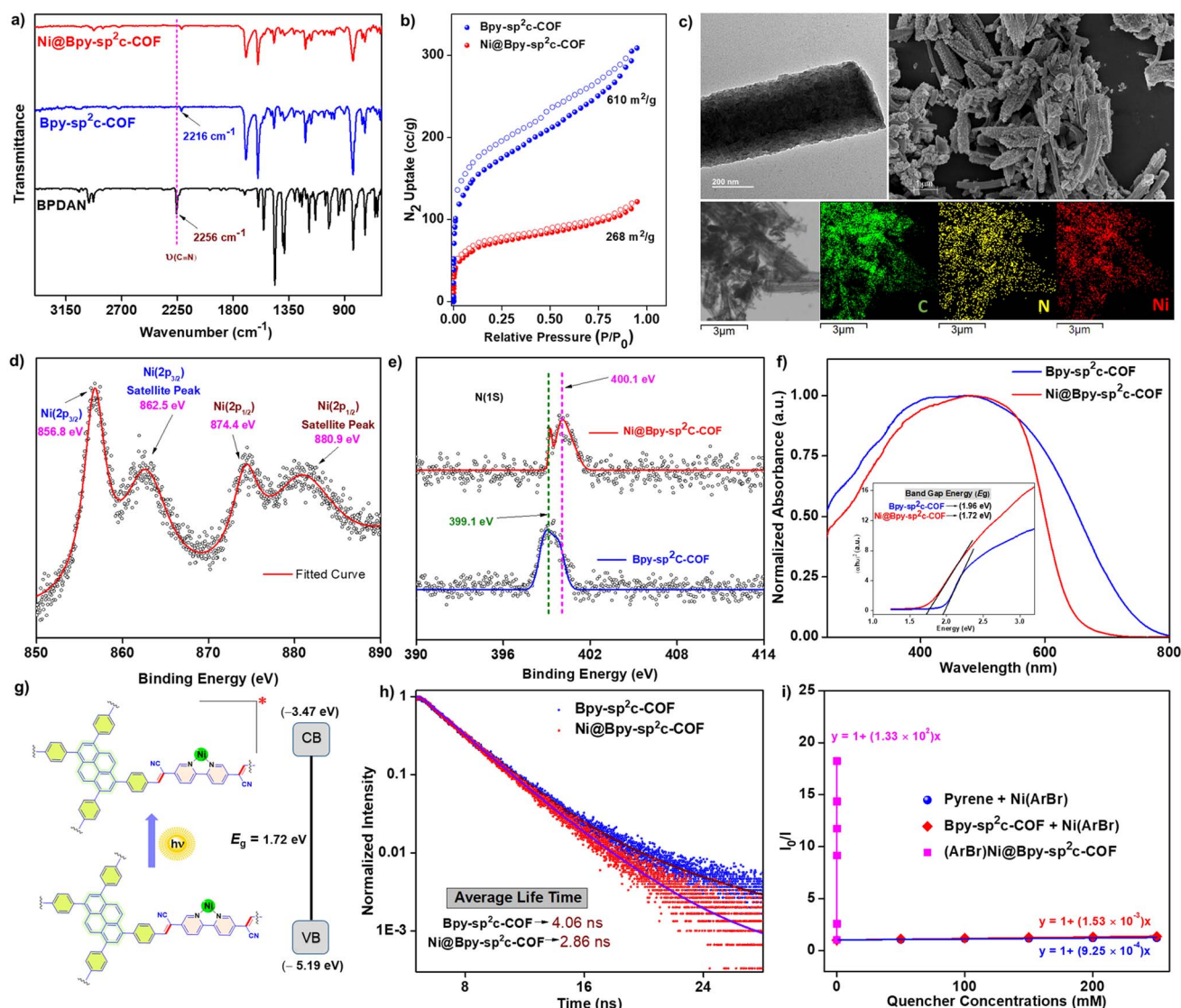
Fig. 2 (a) IR analysis of BPDAN, Bpy- \text{sp}^2\text{c} -COF, and Ni@Bpy- \text{sp}^2\text{c} -COF; (b) BET surface analysis of Bpy- \text{sp}^2\text{c} -COF before and after Ni metal insertion; (c) TEM image (top left corner), SEM image (top right corner), elemental mapping (below) of Ni@Bpy- \text{sp}^2\text{c} -COF; (d) Ni(2p) XPS analysis of Ni@Bpy- \text{sp}^2\text{c} -COF (850 eV to 890 eV region); (e) comparative N(1s) XPS analysis of Bpy- \text{sp}^2\text{c} -COF and Ni@Bpy- \text{sp}^2\text{c} -COF (390 eV to 414 eV region); (f) comparative UV-reflectance spectra and Tauc plot (inset) of Bpy- \text{sp}^2\text{c} -COF and Ni@Bpy- \text{sp}^2\text{c} -COF; (g) the light absorbing ability of Ni@Bpy- \text{sp}^2\text{c} -COF and arrangements of the valence band (VB) and conduction band (CB); (h) average lifetime from time-correlated single-photon counting (TCSPC) experiments; (i) comparative Stern–Volmer photoluminescence quenching for pyrene and Bpy- \text{sp}^2\text{c} -COF by the Ni(ArBr) complex (Ar = 4-CNC 6 H 4 ), and different Ni-loaded Ni(ArBr)@Bpy- \text{sp}^2\text{c} -COF.
