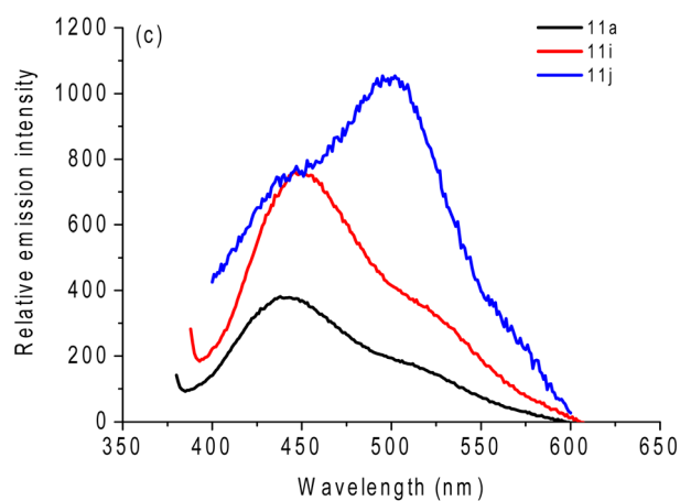
Fig. 4 Comparative steady-state fluorescence emission spectra (concentration at 5.0 \mu M) of compounds 11a (Se atom), 11i (S atom) and 11j (Te atom) in (a) DCM, (b) ACN and (c) DMSO, respectively. The compounds were excited in the higher energy transition band.
