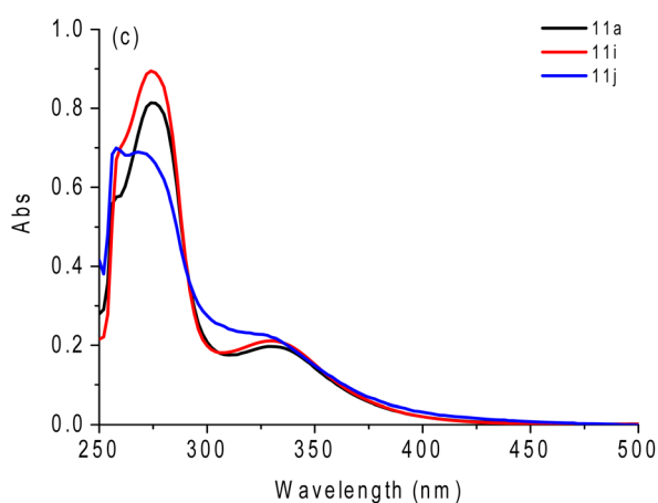
Fig. 3 Comparative absorption UV-vis spectra (concentration at 50 \mu M) of compounds 11a (Se atom), 11i (S atom) and 11j (Te atom) in (a) DCM, (b) ACN and (c) DMSO, respectively.
