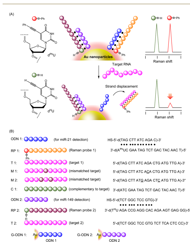
Fig. 1 (A) Schematic illustration of SERS-based detection of multiple nucleic acids targets. When Raman probe (RP: ODNs with alkyne-tag) binds to its corresponding DNA sequence tethered on gold nanoparticles, they show robust SERS signals. When target strand binds with RPs on nanoparticles in a sequence selective manner, the RPs dissociate from the particles, resulting in the decrease of signal intensity. The signal from RPs were changed in the presence of target strands, thereby enabling highly sensitive detection of each target RNA. (B) Sequences of ODNs used in this study.
