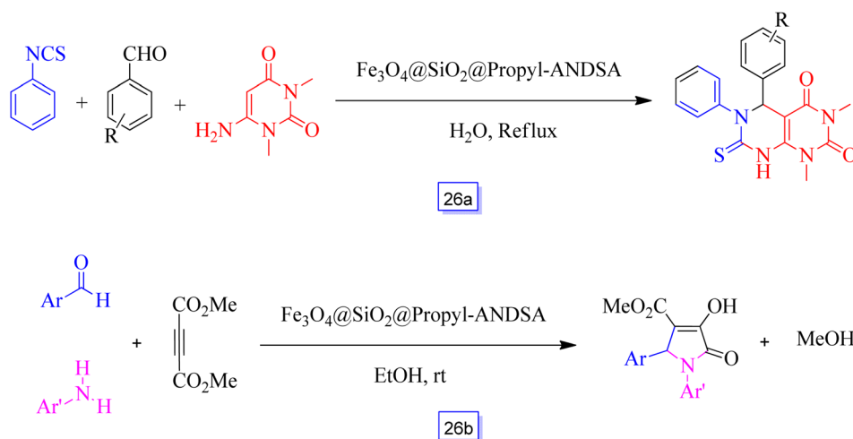
Scheme 26 \text{Fe}_3\text{O}_4@\text{SiO}_2@\text{propyl-ANDSA} catalyzed synthesis of pyrimido[4,5-d]pyrimidine in \text{H}_2\text{O} solvent under reflux condition (a) and general synthesis of polysubstituted 3-hydroxy-2-pyrrolidinones in the presence of \text{Fe}_3\text{O}_4@\text{SiO}_2@\text{propyl-ANDSA} and ethanol solvent at room temperature (b).
