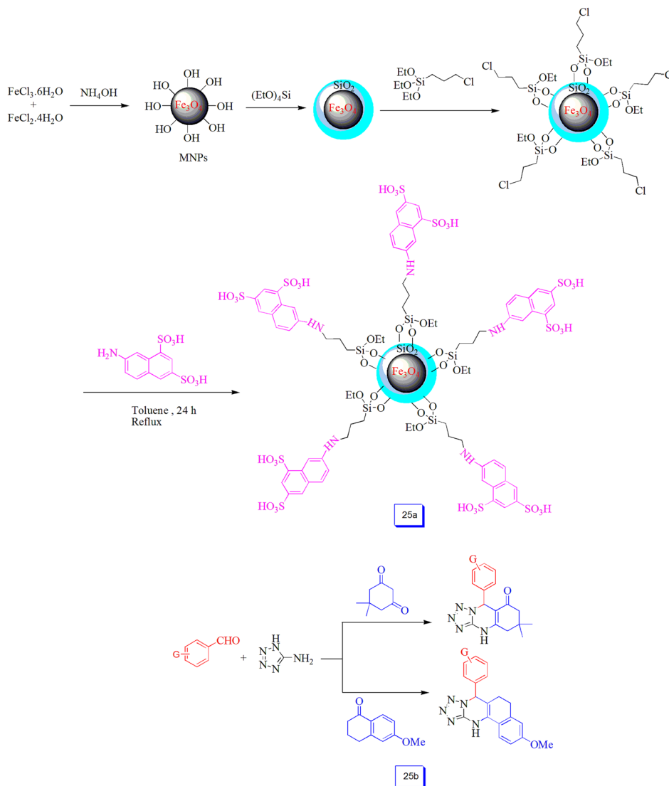
Scheme 25 Stepwise synthesis pathway of \text{Fe}_3\text{O}_4@\text{SiO}_2@\text{propyl-ANDSA} catalyst (a), and one-pot synthesis of tetrahydrotetrazolo[1,5-a]quinazolines and tetrahydrobenzo[h]tetrazolo[5,1-b]quinazolines (b).
