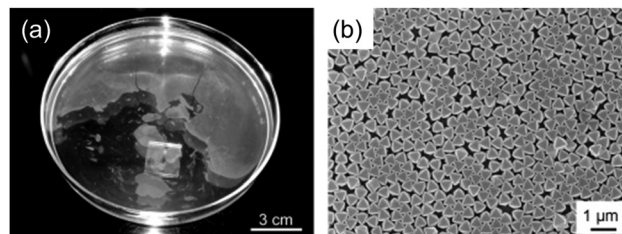
Fig. 15 (a) Photograph and (b) SEM image of aligned 2D monolayer of PVP modified UiO-66 crystals after introduction of SDS solution. Reproduced from ref. 99. Copyright 2013, Wiley-VCH.
