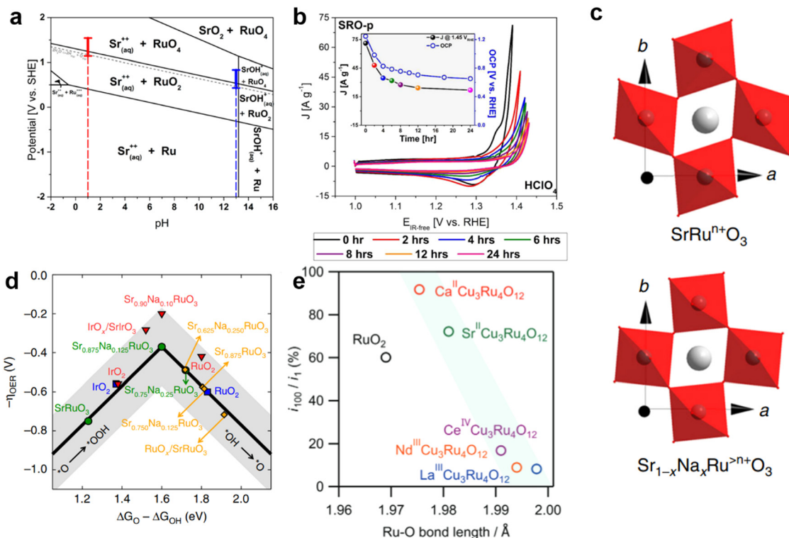
Fig. 11 (a) Pourbaix diagrams of SrRuO 3 . (b) The CV diagram of 10 mV s -1 was performed at 0, 2, 4, 6, 8, 12, and 24 hours after initial contact of the SrRuO 3 with the synthetic air saturated electrolyte in HClO 4 . Reproduced with permission. 61 Copyright 2017, American Chemical Society (c) Diagram of the inhibition of octahedral distortion of SrRuO 3 doped with Na + . (d) The plot of OER Volcano-type activity. Reproduced with permission. 62 Copyright 2019, Springer Nature. (e) A graph showing the relationship between the length of the Ru–O bond and the ratio of current density i_{100}/i_1 at the 100th and 1st cycles. Reproduced with permission. 125 Copyright 2022, Wiley-VCH GmbH.
