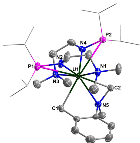
Fig. 5 Molecular structure of 4 with thermal ellipsoids at the 50% probability level. Hydrogen atoms are omitted for clarity. The t Pr groups on P atoms are simplified into lines. Selected bond distances (Å): U1–N1 2.734(4), U1–N2 2.297(3), U1–N3 2.813(4), U1–N4 2.285(4), U1–N5 2.568(3), U1–P1 3.2145(11), U1–P2 3.1286(11), U1–C1 2.553(4), U1–C2 2.461(4).
