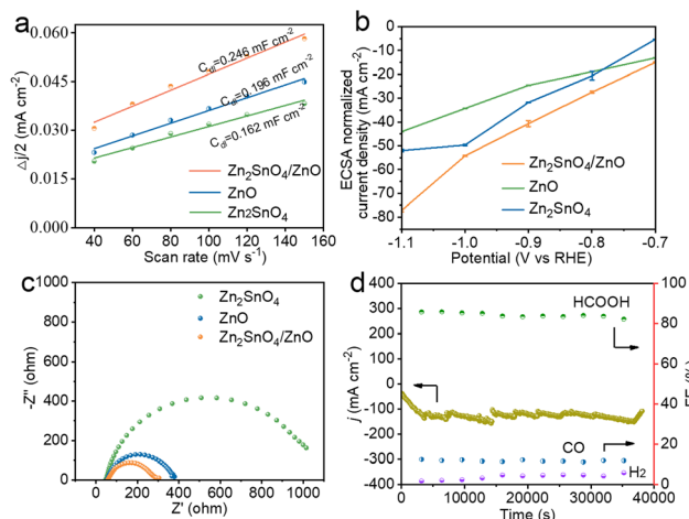
Fig. 6 (a) C dl of Zn 2 SnO 4 /ZnO, Zn 2 SnO 4 and ZnO. (b) ECSA-normalized formate partial current density of Zn 2 SnO 4 /ZnO, Zn 2 SnO 4 and ZnO. (c) Nyquist plots of Zn 2 SnO 4 /ZnO, Zn 2 SnO 4 and ZnO. (d) Stability test on the Zn 2 SnO 4 /ZnO electrode at -1.0 V (vs. RHE).
