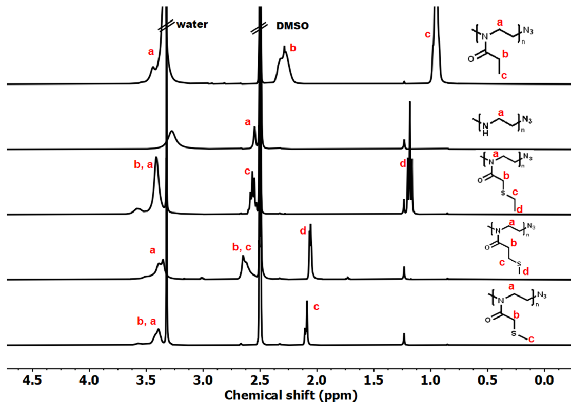
Fig. 1 Representative ^1\text{H} NMR spectra of PETox, PEI, PMTMeOx, PMTtOx, and PETMeOx in \text{DMSO-}d_6 .
