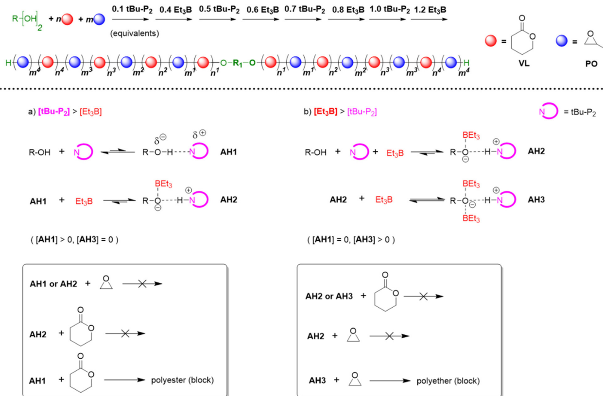
Scheme 10 Top: using the Et_3B /organobase stoichiometry to synthesize well-defined poly(ester-ether) multiblock copolymers. Bottom: different species of activated hydroxyl and respective selectivity.
