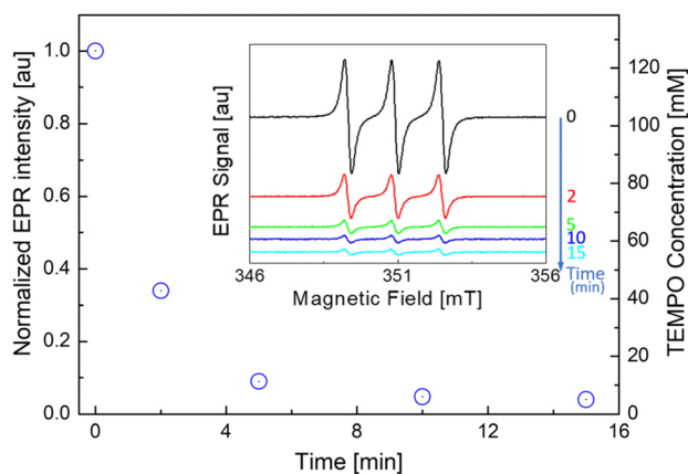
Fig. 4 EPR monitoring of the TEMPO concentration for the reaction of C18 with 4 mol% TEMPO and 2 mol% DCP at 150\text{ }^\circ\text{C} : TEMPO-normalized EPR intensities ( I/I_0 = I(t)/I(t=0) ) were obtained at t = 0, 2, 5, 10 and 15 min with corresponding EPR signals (inset).
