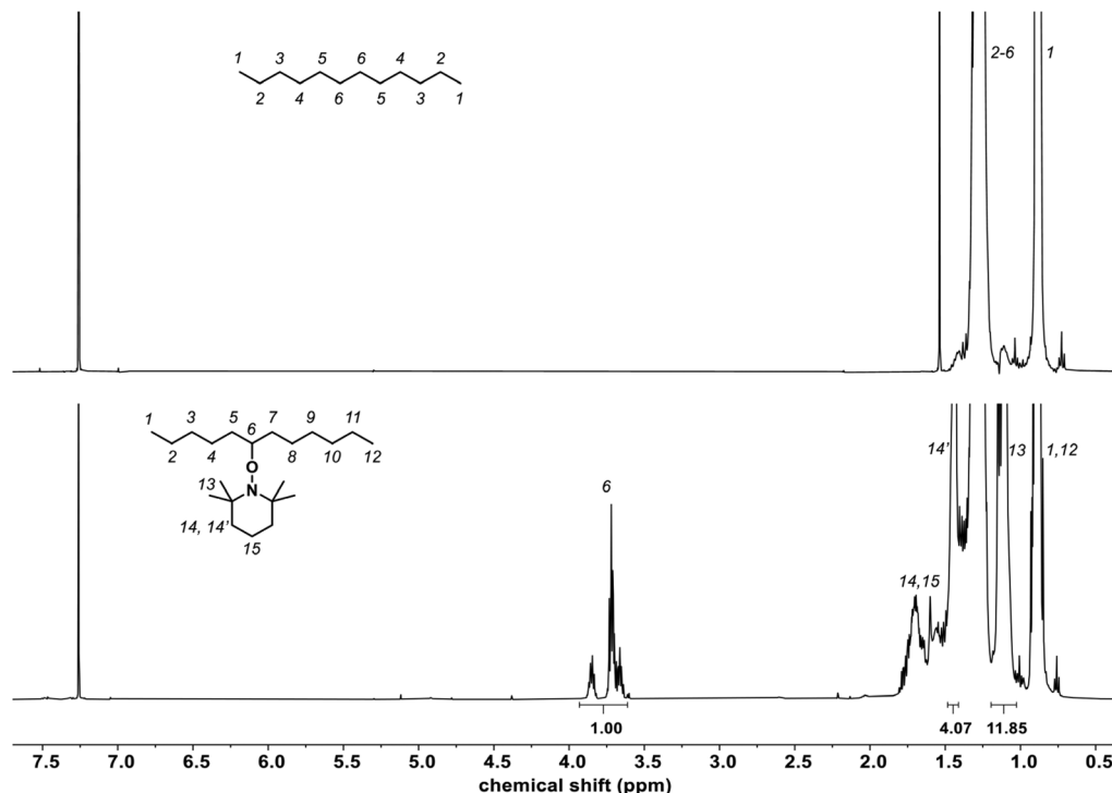
Fig. 3 ^1\text{H} NMR spectra ( \text{CDCl}_3 ) of C12 (top) and TEMPO-grafted C12 (bottom) formed by the reaction of C12 with TEMPO (4 mol%) and DCP (2 mol%) at 150\text{ }^\circ\text{C} after 19 h and concentrated by distillation. The NMR assignment of TEMPO-grafted C12 is illustrated with the TEMPO grafted in the center, but it could be on any carbon of the C12 chain.
