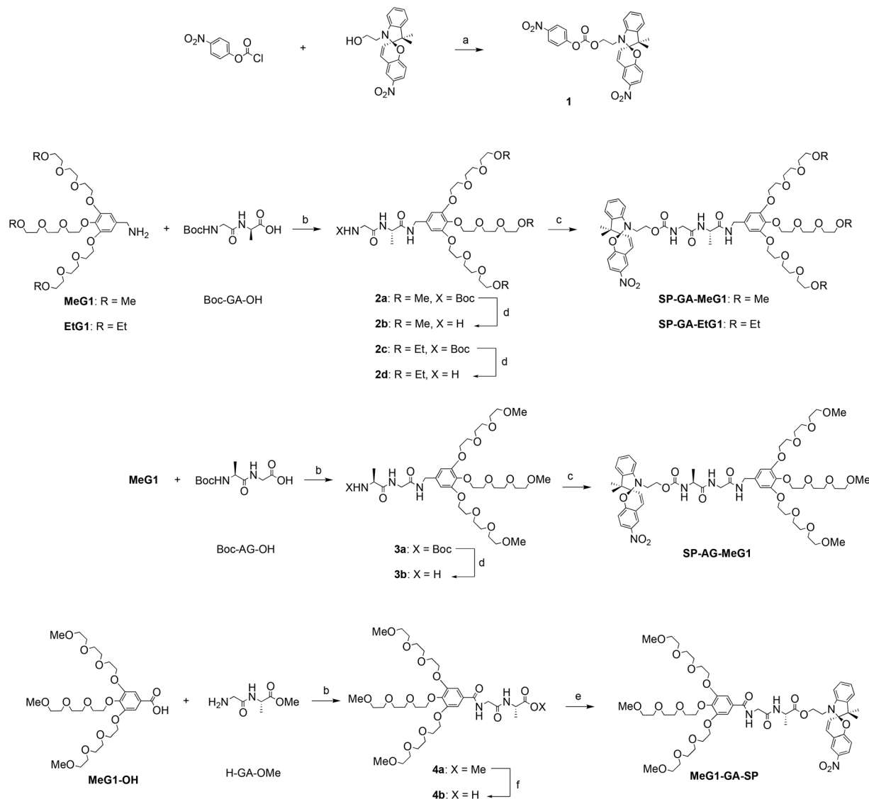
Scheme 1 Synthetic procedure for dendronized spiropyran. Reagents and conditions: (a) DCM, TEA, 0–25 °C, overnight (53%); (b) DCM, HOBT, DiPEA, EDC·HCl, 0–25 °C, overnight (79%); (c) DCM, 1 , TEA, 0–25 °C, overnight (56%); (d) DCM, TFA, 0–25 °C, overnight (100%); (e) 4b , EDC·HCl, DMAP (55%); and (f) MeOH, H 2 O, LiOH·H 2 O, 0–25 °C, overnight (90%). Abbreviations: DCM = dichloromethane, DiPEA = diisopropylethylamine, DMAP = 4-dimethylaminopyridine, EDC·HCl = 1-(3-dimethylaminopropyl)-3-ethylcarbodiimide hydrochloride, HOBT = 1-hydroxy-1H-benzotriazole, TEA = triethylamine, and TFA = trifluoroacetic acid. Abbreviation for amino acids: G for glycine and A for alanine.
