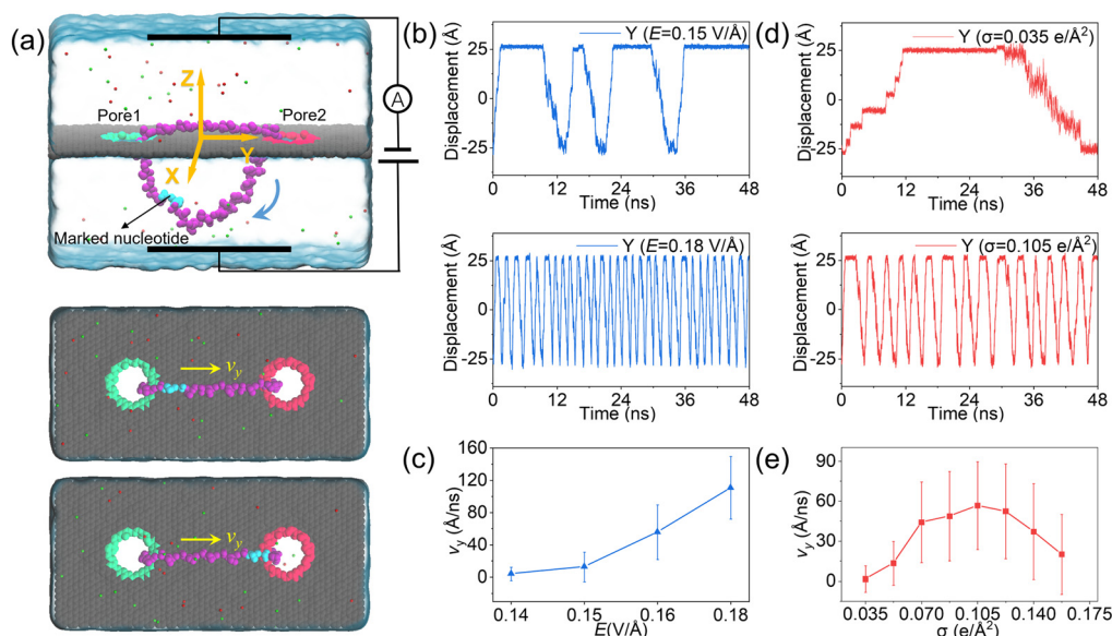
Fig. 2 MD simulations of a circular ssDNA rolling across two independently charged nanopores. (a) Schematic illustration of the simulation setup. The red color and green color of the nanopores indicate that the nanopore is positively and negatively charged, respectively. The blue arrow indicates the rolling direction of the circular ssDNA. Two typical conformations of the circular DNA were also shown below to indicate the two positions where the marked light blue nucleotide is located. (b) The y component of CoM of the marked nucleotide versus simulation time. The displacement traces were shown for the electric fields of 0.15 \text{ V } \text{Å}^{-1} and 0.18 \text{ V } \text{Å}^{-1} as two examples. The two nanopores have the same amplitude of the surface charge density ( 0.105 \text{ e } \text{Å}^{-2} ) but different signs. (c) The effect of external E on the mean sliding velocity of the circular ssDNA along the membrane surface. The velocities (along y direction) of nucleotides within 8 \text{ Å} of the center of the graphene membrane were calculated and averaged using the entire trajectories. (d) The same as panel (b) but for absolute surface charge densities of 0.035 \text{ e } \text{Å}^{-2} and 0.105 \text{ e } \text{Å}^{-2} , respectively. The electric field was 0.16 \text{ V } \text{Å}^{-1} . (e) The same as panel (c) but for the effect of \sigma on the mean sliding velocity of the circular ssDNA along the membrane surface.
