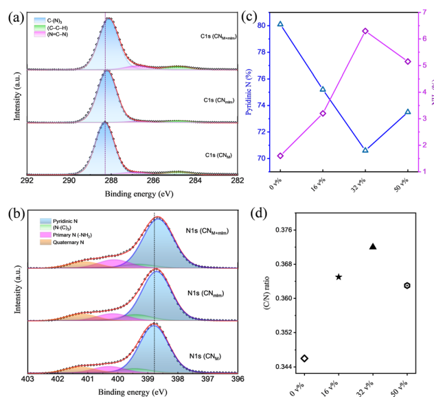
Fig. 4 XPS CN analysis. High-resolution (a) C 1s and (b) N 1s XPS spectra of CN M , CN M+mlm , and CN M+mlm . (c) Calculated percentage of pyridinic N and free NH 2 species for various amounts of EG (v%) used in the hydrothermal treatment during CN M+mlm syntheses, calculated from N 1s spectra. (d) Atomic C/N ratio obtained from survey scans of CN M+mlm prepared with varying EG content. The experimental points in (a) and (b) are fitted with a red line, which is deconvoluted into peaks corresponding to the indicated chemical species. The lines connecting the diamonds and triangles in (c) serve as a guide to the eye.
