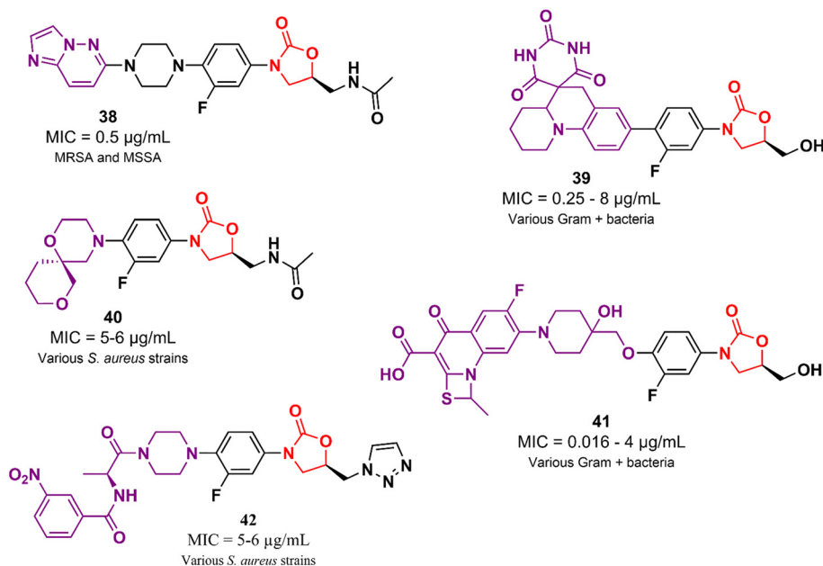
Fig. 8 Antibacterial agents containing the oxazolidinone scaffold as the pharmacophore.
