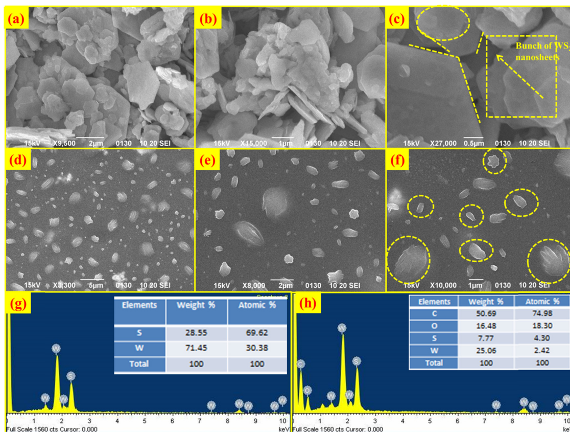
Fig. 2 Scanning electron micrographs of WS 2 nanosheets at (a) 2 \mu m, (b) 1 \mu m and (c) 0.5 \mu m, scanning electron micrographs of WS 2 nanosheets embedded in a PVOH matrix at (d) 5 \mu m, (e) 2 \mu m and (f) 1 \mu m, (g) EDS spectrum of WS 2 nanosheets and (h) EDS spectrum of WS 2 PVOH.
