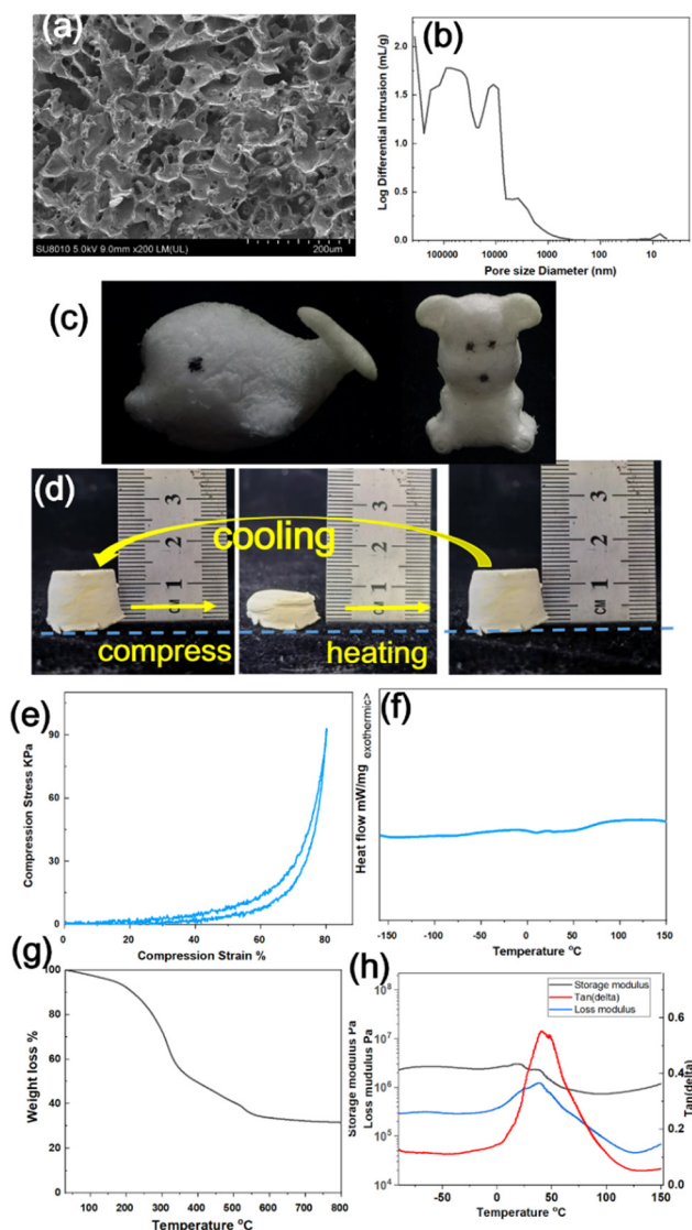
Fig. 1 (a) SEM image, and (b) pore size distribution obtained by mercury porosimetry of the SS-COOH. (c) The sponge whale and bear; (d) the shape memory property photograph of the SS-COOH before and after compression at room temperature and heating at 90 ^{\circ}\text{C} after about 1 min. (e) Compressive stress-strain curve under 80% strain of the SS-COOH at 90 ^{\circ}\text{C} . (f) DSC curve from -150 to 150 ^{\circ}\text{C} under \text{N}_2 at 10 ^{\circ}\text{C min}^{-1} of the SS-COOH and (g) TGA curves of SS-COOH under air at 10 ^{\circ}\text{C min}^{-1} . (h) DMA curve of the SS-COOH.
