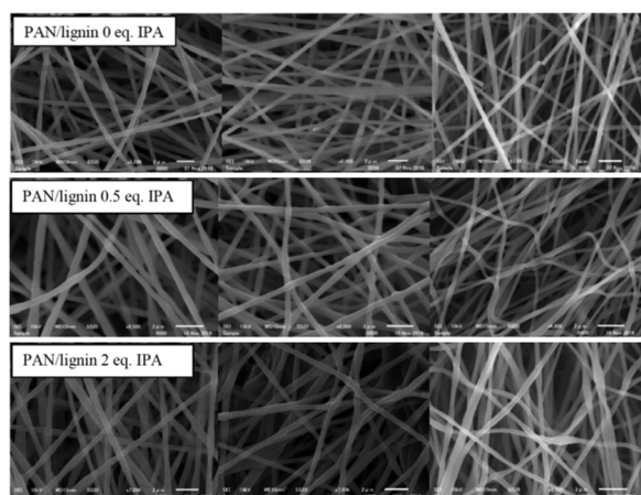
Fig. 9 SEM images of electrospun fibers (left), after thermostabilization (middle; T = 250^\circ\text{C} for t = 1 h at 0.5^\circ\text{C min}^{-1} ), and carbonization (right; T = 1000^\circ\text{C} at 5^\circ\text{C min}^{-1} ) steps using acetylated lignin with different amounts of iPAc and s-OH. Adapted with permission from ref. 178. Copyright 2021 Elsevier Ltd.
