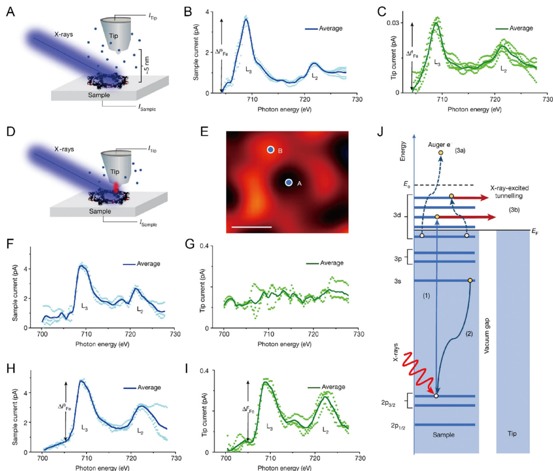
Fig. 3 (A) Schematic of SX-STMs in the far-field regime. (B) STM-XAS spectra of the sample current. (C) STM-XAS spectra of the tip current. (D) Schematic of SX-STMs in the tunnelling regime. (E) STM image of a single supramolecular ring measured with the SX-STMs setup. (F–I) Simultaneously recorded STM-XAS spectra of the sample and tip channels in the tunnelling regime when the tip is on position A (F) and (G) and when the tip is on position B (H,I). (J) X-Ray-excited electron tunnelling process. Reproduced with permission. 36 Copyright © 2023, Springer Nature.
