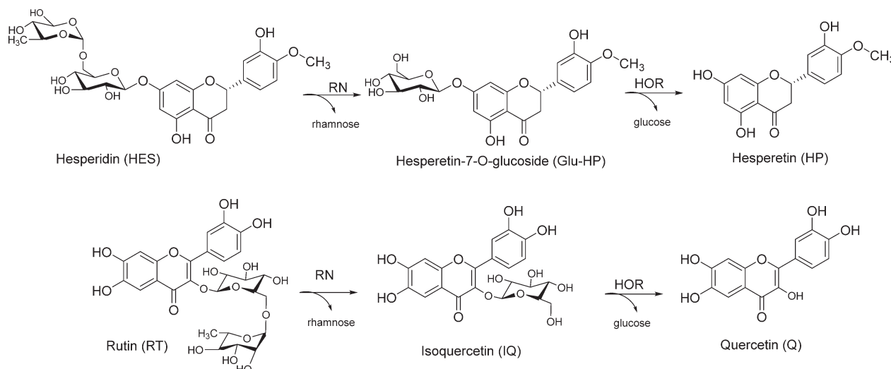
Scheme 1 Obtainment of quercetin and hesperetin as aglycones from the corresponding natural rutinosides.
