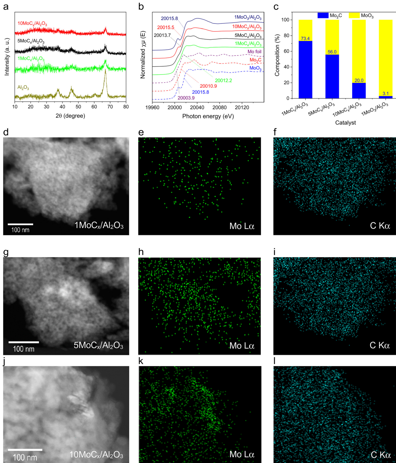
Fig. 3 (a) XRD patterns of Al_2O_3 and tested catalysts, (b) XAS spectra, and (c) linear combination fitting (LCF) results of supported MoC_x catalysts. MoO_3 , Mo_2C , Mo foil, and 1 MoO_3 /Al _2 O _3 were included as the standards. Representative dark-field TEM images of (d) 1 MoC_x /Al _2 O _3 , (g) 5 MoC_x /Al _2 O _3 , and (j) 10 MoC_x /Al _2 O _3 and their EDS mapping results at Mo L \alpha and C K \alpha . (e) and (f) show the EDS mappings of 1 MoC_x /Al _2 O _3 ; (h) and (i) 5 MoC_x /Al _2 O _3 ; (k) and (l) 10 MoC_x /Al _2 O _3 .
