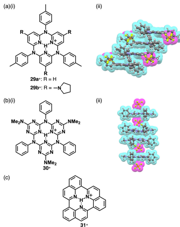
Fig. 19 (a) (i) Protonated azacalix[3](2,6)pyridine 29\text{a,b}^+ and (ii) single-crystal X-ray structure of 29\text{a}^+-\text{PF}_6^- (redrawn from a cif file: 298963), (b) (i) protonated azacalix[3]triazine 30^+ and (ii) single-crystal X-ray structure of 30^+-\text{PF}_6^- (redrawn from a cif file: 2072959) and (c) protonated triquinoline 31^+ .
