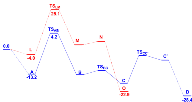
We also performed an energy decomposition analysis (EDA) 19 using the ADF program 20 (see the Computational details section and Table S2 in the ESI † ). The binding energy (BE) of QO to the PdCl 2 fragment is -36.7 and -28.4 kcal mol -1 in A and L , respectively. The interaction energies, \Delta E_{\text{int}} ( -51.6 ( A ) and -38.7 ( L ) kcal mol -1 ), differ from the BE by the preparation energy of the fragments, due to the change in geometry when the optimized fragment is in the molecule ( \Delta E_{\text{prep}} ). These energies differ by 4.6 kcal mol -1 and are larger (more destabilizing) for A . Among the other terms, the preference for \sigma coordination ( A ) can be assigned to a much larger electrostatic interaction ( -126.9 and -91.2 kcal mol -1 , respectively for A and L ), which is not compensated by the smaller Pauli repulsion term and more attractive orbital interaction in L . Solvent effects are negligible.
