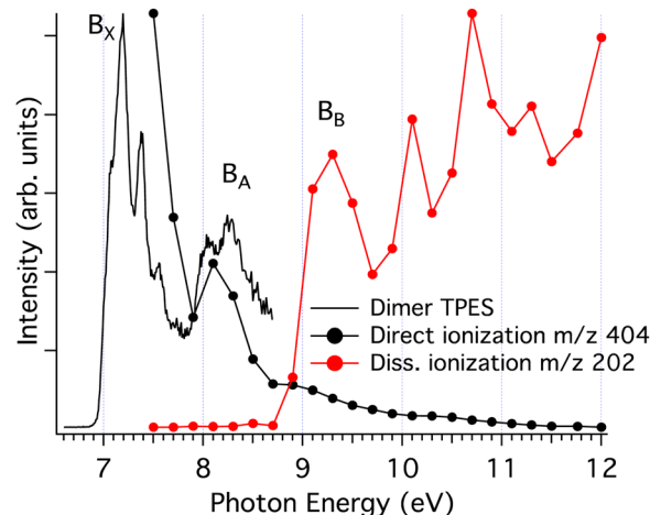
Fig. 6 Threshold photoelectron spectrum showing the vibronic states of the pyrene dimer 10 (black curve). The black circles show the threshold photoelectron signal corresponding to direct ionisation of the parent dimer with an energy resolution of 300 meV, obtained by considering only ions having very low translational energies (<20 meV). The red circles show the threshold photoelectron signal corresponding to dissociative ionisation into the monomer channel, obtained with an energy resolution of 300 meV. The experimental bands, B, relevant for the discussion have been labelled.
