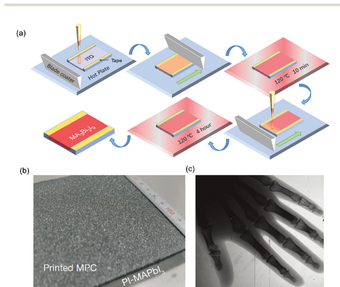
Fig. 5 Blade coating method. (a) Schematic diagram of blade coating. (b) Printed \text{MAPbI}_3 film. 80 (c) Hand skeleton image by the \text{MAPbI}_3 detector. Reproduced with permission. 63 Copyright 2017, Springer Nature.
