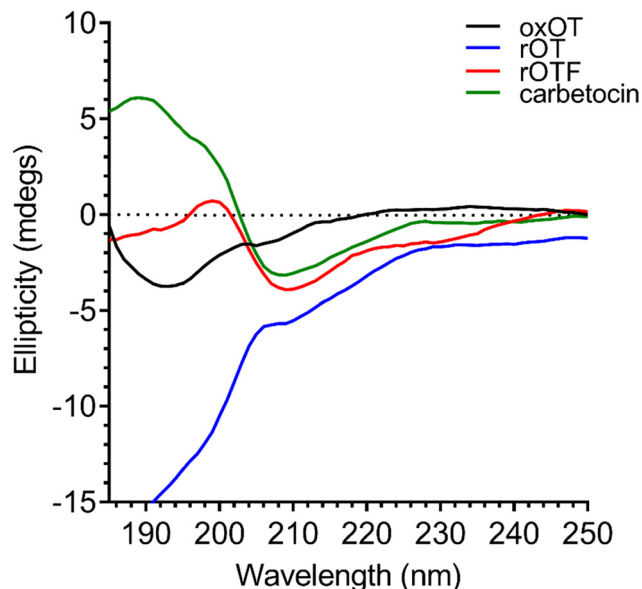
Fig. 2 Circular dichroism spectra of 40 μM oxOT, rOT, rOTF, and carbetocin (15 mM phosphate, pH 7.4).
