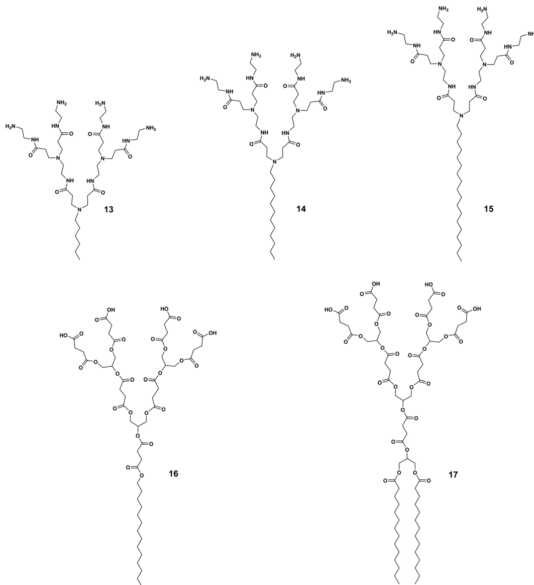
Fig. 4 Impact of hydrophobic chain length and number on the balance between antibacterial activity and toxicity as demonstrated by the amphoteric dendrimers 13 , 14 , 15 , 16 and 17 .
