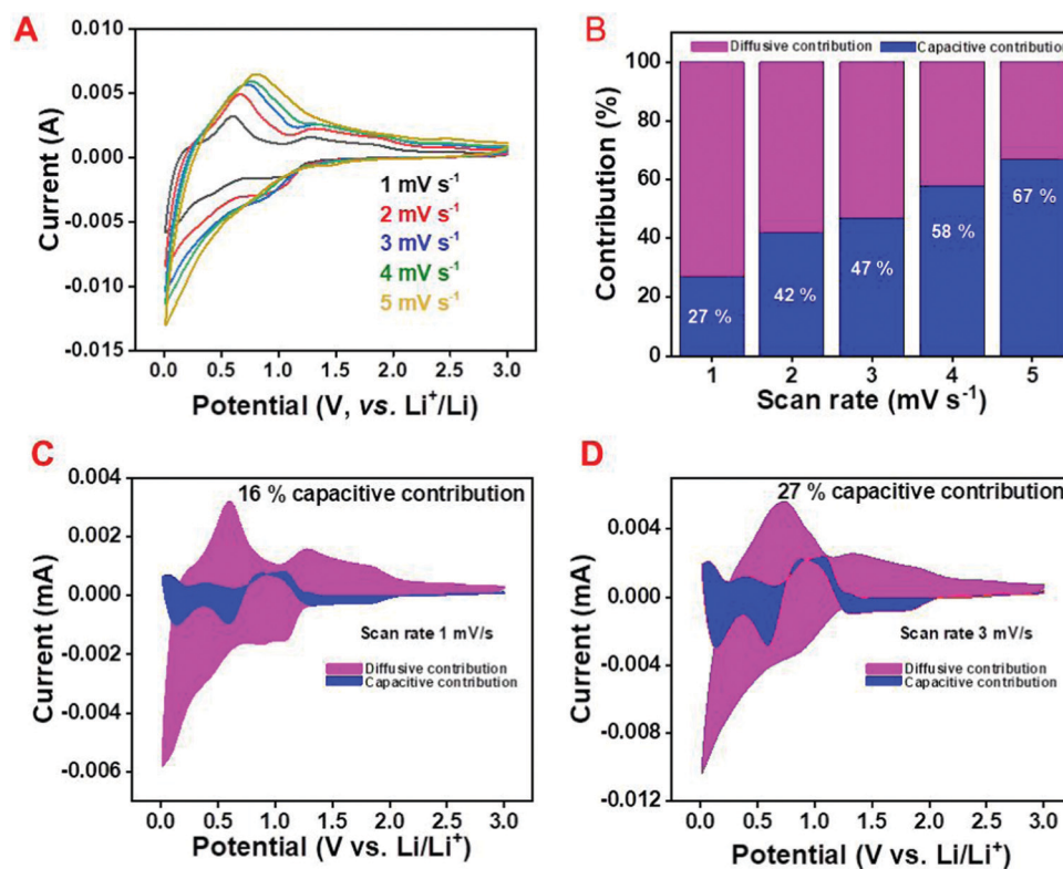
Fig. 4 Kinetics of the Li-ion in the \text{C/SnO}_2 composite; (A) cyclic voltammogram curve, (B) capacitive and diffusive contribution curve at different scan rates for a fixed potential (at 0.58 \text{ V} ), and capacitive and diffusive contribution in a cyclic voltammogram curve for a fixed scan rate, (C) 1 \text{ mV s}^{-1} and (D) 3 \text{ mV s}^{-1} .
