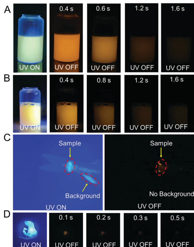
Fig. 7 (A) and (B) Photographs of (A) \text{N}\beta\text{NBF}_2 -MeOBP-0.5% and (B) \text{N}\beta\text{NBF}_2 -MeOBP-0.5% + R6G afterglow dispersion under 365 nm UV light and after removal of the UV light. (C) and (D) Preliminary bioimaging studies of the \text{N}\beta\text{NBF}_2 -MeOBP-0.5% afterglow dispersion in living (C) fish and (D) mice.
