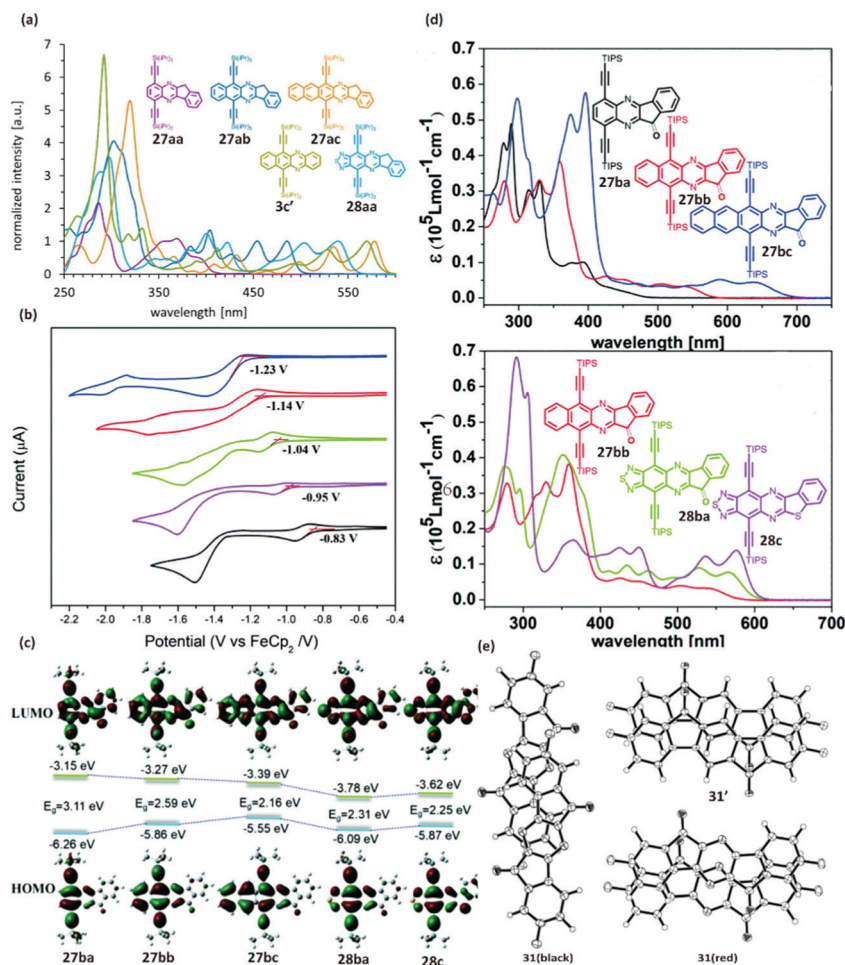
Fig. 6 (a) Normalized (lowest-energy maximum) absorption spectra of 27aa–27ac , 28aa and 3c' in n -hexane. (b) CV of 27ba–27bc , 27bb , 28ba , and 28c in CH 2 Cl 2 and 0.1 M Bu 4 NPF 6 on a Pt electrode at a scan rate of 50 mV s -1 vs. Ag/AgCl wire. (c and d) Absorption spectra and frontier molecular orbital diagram of 27ba–27bc (upper) and 27bb , 28ba , and 28c (bottom) in CH 2 Cl 2 . (e) Packing structures of 31 (black, left; red, right, bottom) and 31' (right, upper) in single crystals. (a) was reproduced with permission from ref. 70. Copyright 2016, American Chemical Society. (b, c, and d) were reproduced with permission from ref. 53. Copyright 2019, Royal Society of Chemistry. (e) was reproduced with permission from ref. 74. Copyright 2008, American Chemical Society.
