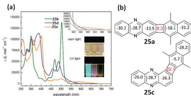
Fig. 4 (a) UV-Vis absorption spectra of 25b, 25d, and 25e in \text{CHCl}_3 . The inserted photographs are the dilute solutions of 25b, 25d, and 25e (from left to right) under room light and 365 nm UV irradiation. (b) NICS ( 1 ) _{\pi,\text{ZZ}} calculations on 25a and 25c. Reproduced with permission from ref. 26. Copyright 2018, American Chemical Society.
