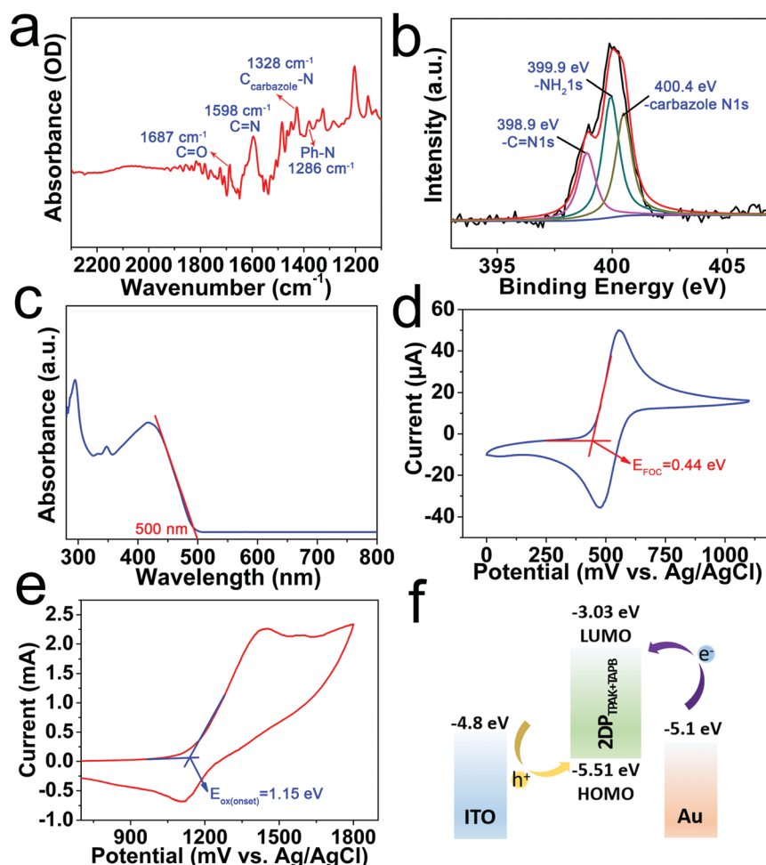
Fig. 2 (a) IR spectra of 2DP_{TPAK+TAPB} . (b) XPS N 1s spectra of 2DP_{TPAK+TAPB} . (c) UV-Vis spectra of the 2DP_{TPAK+TAPB} film ( E_{\text{eg}} = hc/\lambda = 1240/500 = 2.48 eV). (d) and (e) CV curve of the ferrocene standard and 2DP_{TPAK+TAPB} film. The CV curve of the ferrocene standard, swept under the same conditions as for the film. E_{\text{FOC}} was measured to be 0.44 eV vs. Ag/AgCl in \text{CH}_3\text{CN} . E_{\text{HOMO}} = -[E_{\text{ox(onset) vs. Ag/AgCl}} + 4.8 - E_{\text{FOC}}] = -5.51 eV; E_{\text{LUMO}} = E_{\text{HOMO}} + E_{\text{eg}} = -3.03 eV. (f) Schematic energy diagram of an Au/ 2DP /ITO structure.
