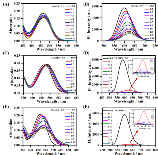
Fig. 2 The absorption (A, C and E) and fluorescence (B, D and F) spectra of LDER in 1,4-dioxane-ethyl acetate, toluene-DMSO and 1,4-dioxane- \text{H}_2\text{O} mixtures with different volume ratios; inset: the enlarged part indicated by the red arrow. Concentration = 10 \mu M.
