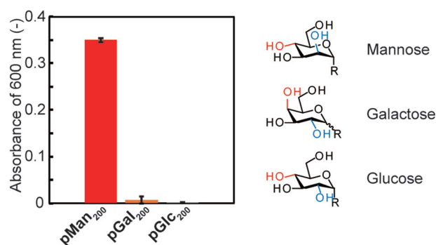
Fig. 4 Turbidity measurement of pMan 200 , pGal 200 and pGlc 200 and the chemical structure of monosaccharides. Turbidity of each glycopolymer was measured after dissolution in HEPES buffer at 1 g L^{-1} and standing at 15^\circ C for 48 h.
