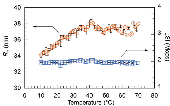
Fig. 6 Hydrodynamic radius ( R_h , ○) and light scattering intensity (LSI, □) of C_{70} /EUM at C_p = 2 \text{ g L}^{-1} and [C_{70}]_s = 0.313 \text{ g L}^{-1} in PBS as a function of temperature.
