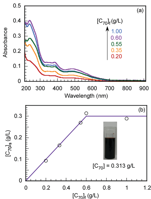
Fig. 3 (a) UV-vis absorption spectra of C 70 /EUM at C_p = 2 g L -1 and (b) the amount of solubilized C 70 in PBS ( [C_{70}]_s ) as a function of the amount of C 70 ( [C_{70}]_f ) used.
