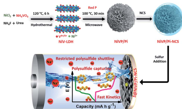
Scheme 1 Schematic representation of the synthetic protocol of NiVP/Pi-NCS and redox conversion of polysulfide at S@NiVP/Pi-NCS anode in aqueous Na-ion/S battery.
