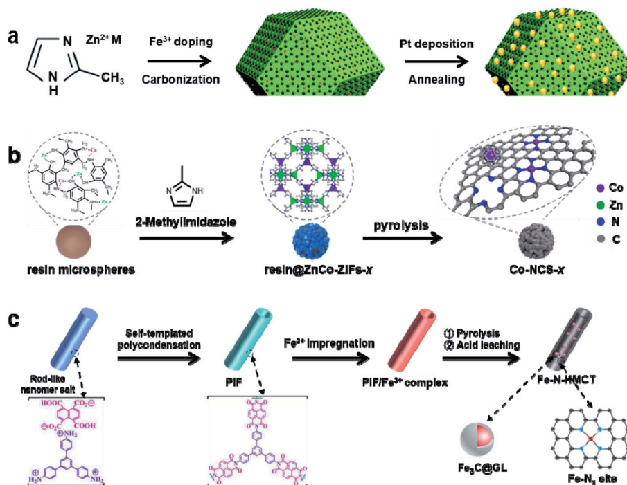
Fig. 2 (a) Synthesis scheme of the FeN 4 -C derived carbon-supported Pt or PtCo catalysts. Reproduced from ref. 37 with permission from the Royal Society of Chemistry, copyright 2021. (b) Schematic illustration of the synthesis process of Co-NCS-x. Reproduced from ref. 40 with permission from Elsevier Ltd, Copyright 2021. (c) Schematic illustration for the synthesis of Fe-N-HMCT catalysts. Reproduced from ref. 42 with permission from Wiley-VCH GmbH, copyright 2020.
