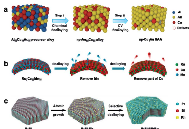
Fig. 6 Dealloying method: (a) schematic illustration for the preparation of np-Cu 1 Au SAA with surface defects. Reproduced from ref. 65 with permission from Science China Press and Springer-Verlag GmbH Germany, copyright 2021. (b) Schematic illustration of the preparation procedure of np-Cu 100-x Ru x . Reproduced from ref. 66 with permission from the American Chemical Society, copyright 2020. (c) Schematic illustration of the preparation procedure of PtBi-3.6% Rh 1 and PtBi@PtRh 1 nanoplates. Reproduced from ref. 67 with permission from Wiley-VCH GmbH, copyright 2021.
