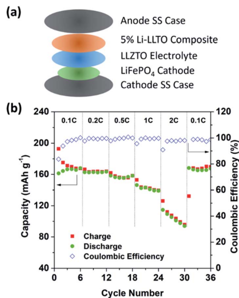
Fig. 7 The overall SSB cycling performance. (a) Assembly of the solid-state lithium batteries. (b) Performance of the \text{LiFePO}_4|\text{LLZTO}|\text{Li-LLTO} solid-state cells at different charge–discharge rates.
