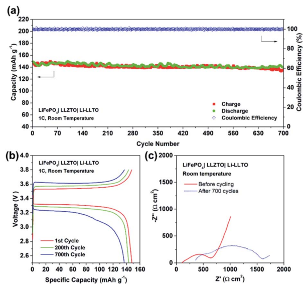
Fig. 8 The overall SSB cycling performance. (a) Cycling performance of \text{LiFePO}_4|\text{LLZTO}|\text{Li-LLTO} at a rate of 1C at room temperature. (b) Charge and discharge curves for the 1 st , 200 th , and 700 th cycles at 1C. (c) EIS curves of the fresh cell and cycled cell for the \text{LiFePO}_4|\text{LLZTO}|\text{Li-LLTO} SSB.
