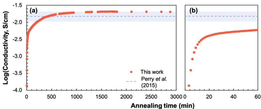
Fig. 10 Plot of conductivity over the full annealing period (a) and over the first hour (b) at 400 °C in \sim 0.2 atm UHP O_2 and \sim 0.8 atm UHP Ar; dashed line shows the conductivity and conservative uncertainty estimate (shaded blue) of a crystalline-grown STF35 thin film 26 under the same conditions.
