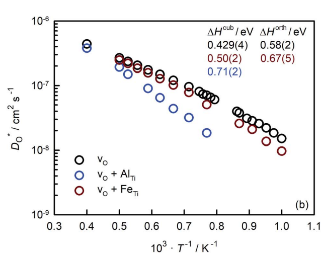
Fig. 5 Tracer diffusion coefficients of oxygen obtained for \text{CaTiO}_3 with oxygen vacancies and charge-compensating acceptor-type defects: (a) native acceptor defects, (b) foreign acceptor defects. In all cases, the site fraction of oxygen vacancies was n_v = 0.2\% .
