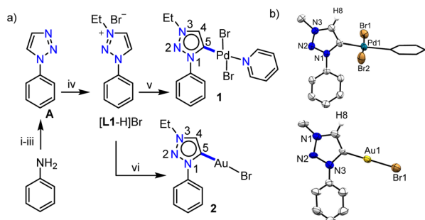
Scheme 1 (a) Synthesis of [\text{L1-H}]\text{Br} and its palladium ( 1 ) and gold ( 2 ) complexes: (i) \text{NaNO}_2 , \text{HCl}/\text{H}_2\text{O} (10% solution), 0^\circ\text{C} , 1 h; (ii) \text{NaN}_3 , 0^\circ\text{C} –RT, 12 h; (iii) vinyl acetate, reflux, 24 h; (iv) \text{EtBr} , \text{CH}_3\text{CN} , reflux, 24 h; (v) [\text{Pd}(\text{CH}_3\text{CN})_2\text{Cl}_2] , \text{Cs}_2\text{CO}_3 , \text{KBr} , \text{CH}_3\text{CN}/\text{pyridine} , 70^\circ\text{C} , 24 h; (vi) [\text{Au}(\text{SMe}_2)\text{Cl}] , \text{Cs}_2\text{CO}_3 , \text{CH}_3\text{CN} , 70^\circ\text{C} , 24 h; (b) molecular structures of 1 and 2 with ellipsoids at a 50% probability level. Hydrogen atoms except H8 and Me moieties of the N-Et groups are omitted for clarity. Pyridine is shown in capped stick.
