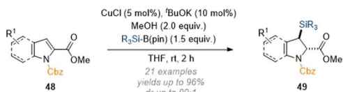
Scheme 15 C-3 silylation of indoles using copper catalysis. 20
