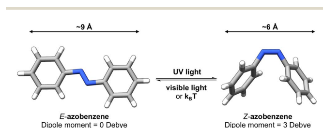
Fig. 1 Photoswitchable molecules undergo reversible structural changes between multiple states upon irradiation with light.
