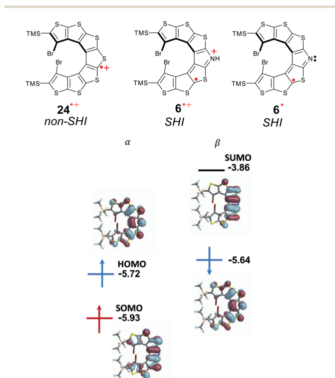
Fig. 16 Chemical structures of cationic radicals thia[7]helicene 24^{+\bullet}[\text{PF}_6]^{-} and aza-thia[7]helicene 6^{+\bullet}[\text{PF}_6]^{-} , and neutral aza-thia[7]helicene 6^{\bullet} . Orbital energies (in eV) and isosurfaces ( \pm 0.030 \text{ a.u.} ) of selected MOs of 7^{\bullet} . Figures adapted with permission from ref. 53. Copyright 2021 American Chemical Society.
