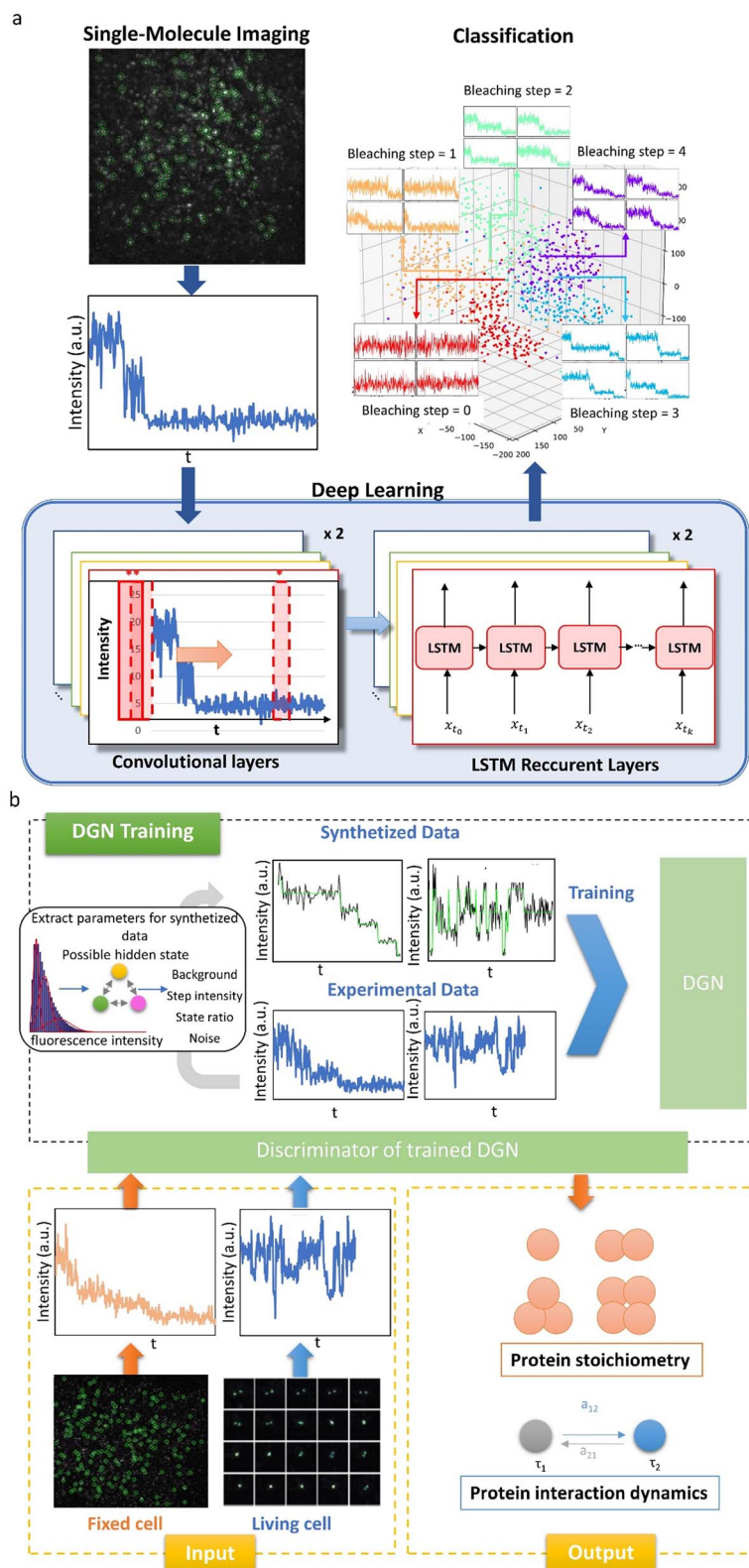
Fig. 3 Deep learning for single molecule stoichiometry studies. (a) Architecture of the CLDNN for SMPSA. 16 Copyright © 2019, American Chemical Society. (b) The training and performances of the DGN on both SMPSA and dynamic finding with fluorescence intensity traces. 100 Copyright © 2020, The Author(s).
