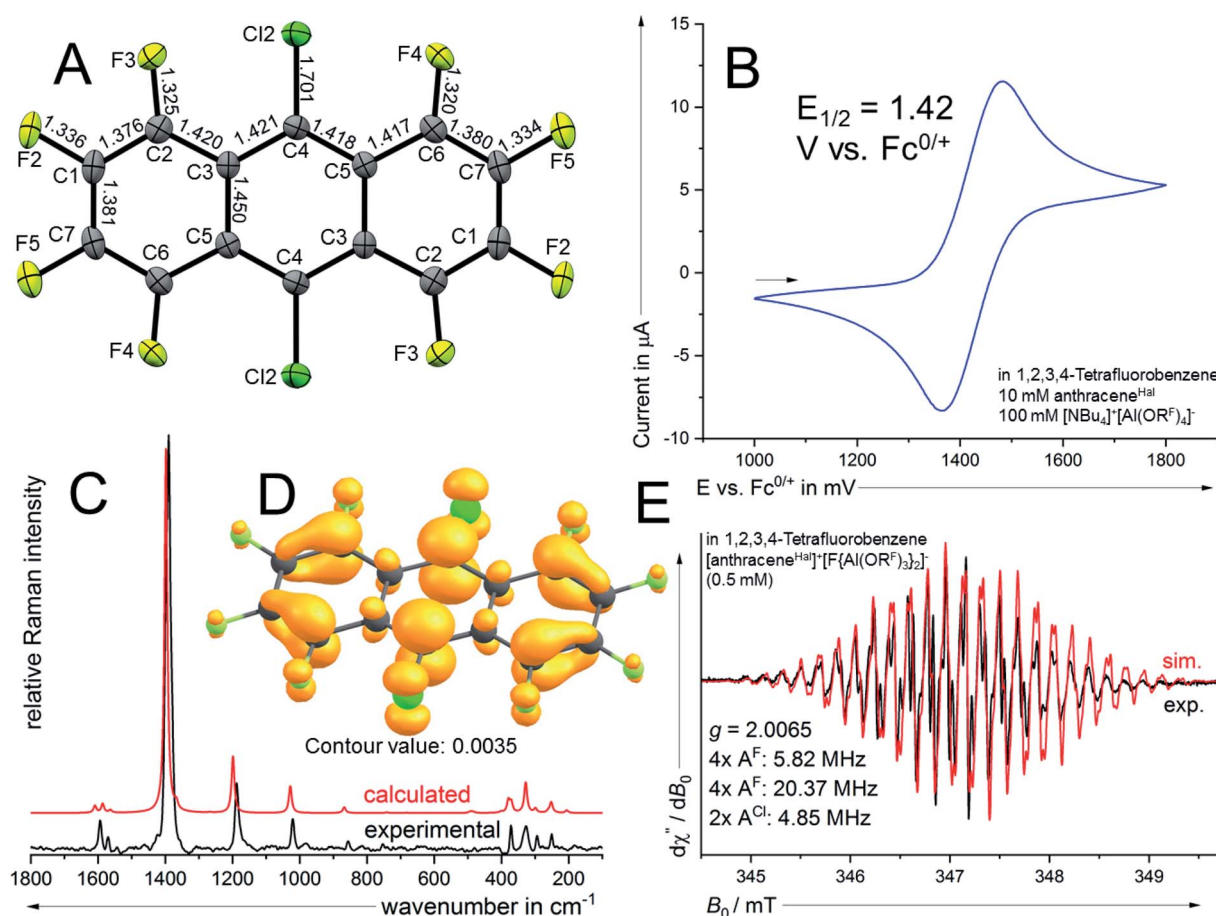
Fig. 4 (A) Molecular structure of the radical cation in [\mathbf{6}]^{+\bullet}[\text{F}\{\text{Al}(\text{OR}^F)_3\}_2]^- (ellipsoids set at 50% probability, distances in Å and standard deviations of the C–C bonds in the range of 0.003 Å). Colour code: carbon – grey, fluorine – light green, chlorine – dark green. (B) Cyclovoltammetry ( 2^{\text{nd}} cycle; 100 \text{ mV s}^{-1} ) of 6 . (C) calculated (B3LYP(D3BJ)/def2-TZVPP) Raman spectrum of [\mathbf{6}]^{+\bullet} and experimental Raman spectrum of crystalline [\mathbf{6}]^{+\bullet}[\text{F}\{\text{Al}(\text{OR}^F)_3\}_2]^- . (D) Spin density plot (B3LYP(D3BJ)/def2-TZVPP) of [\mathbf{6a}]^{+\bullet} . (E) EPR spectrum of a 0.5 mM solution of [\mathbf{6}]^{+\bullet}[\text{F}\{\text{Al}(\text{OR}^F)_3\}_2]^- in TFB and simulated EPR spectrum using the hyperfine coupling constants indicated in the figure.
